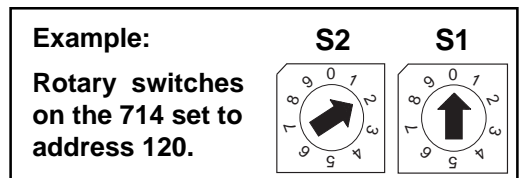
Figure 2: Address switch settings
